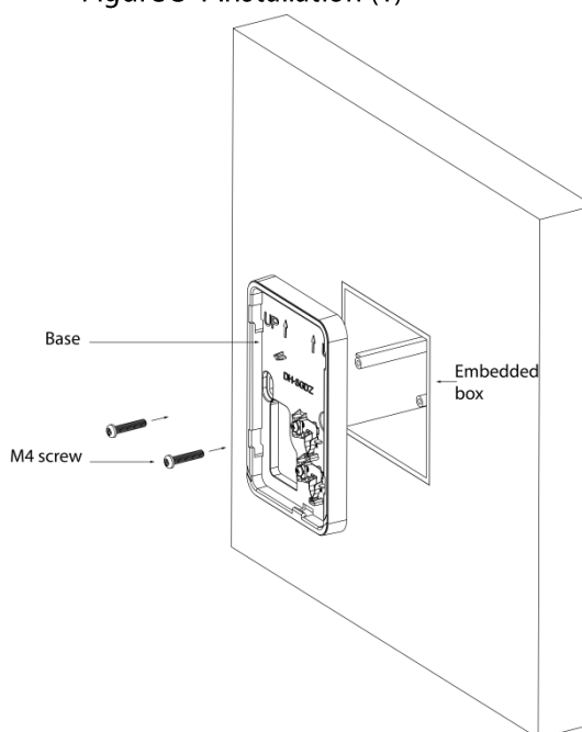
Figure 3-1 Installation (1)
