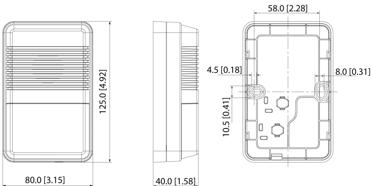
Figure 1-1 Dimensions (mm[inch])
