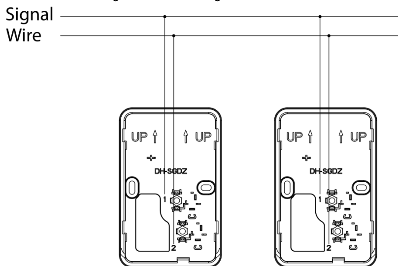
Figure 3-3 Installation (2)
